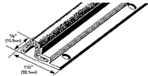
DS422 Extruded Aluminum Brown or White Enamel Paint with Matching Brown or White Foam-Tight compression gasket. Clear Anodized Insert is Black
