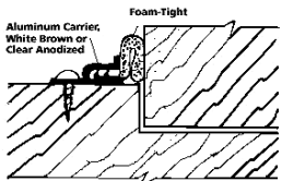
DS422 Extruded Aluminum Brown or White Enamel Paint with Matching Brown or White Foam-Tight compression gasket. Clear Anodized Insert is Black
